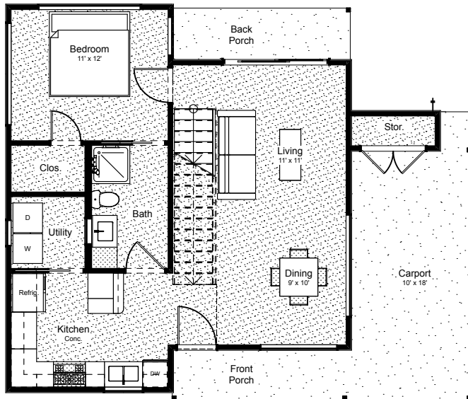
Lower Floor Area A: 746 sq ft
