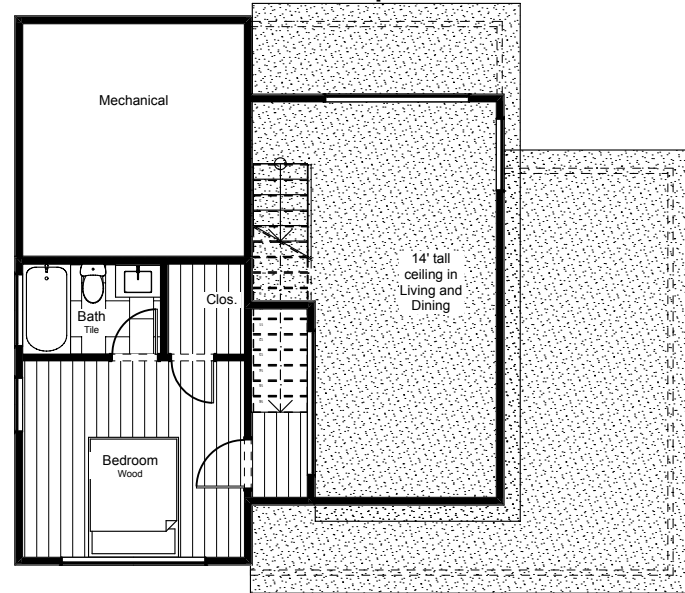
Second Floor Area A: 265 sq ft
