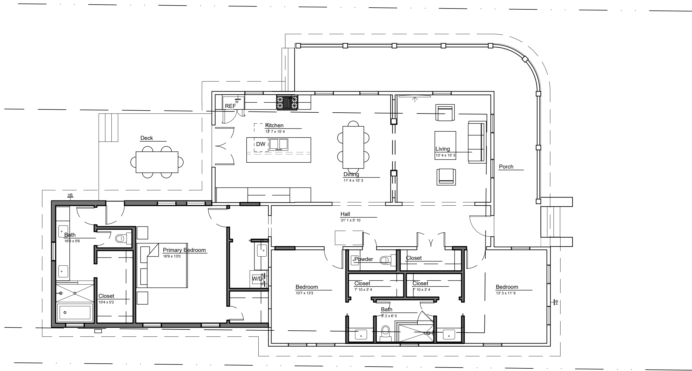
Level 1 Plan
